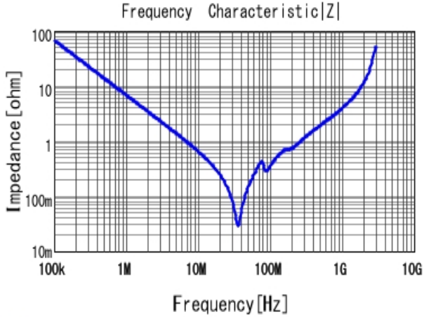
■ GA355DR7GB223KW01 |Z| DCOV, 25degC
