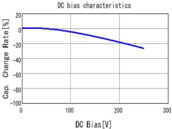
■ GA355DR7GB223KW01 C-DC bias capchange, 25.0degC, AC1V
