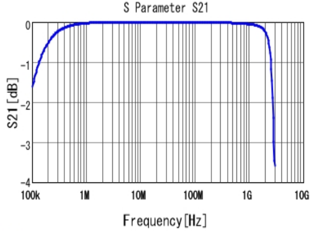
■ GA355DR7GB223KW01 S21 DCOV, 25degC
