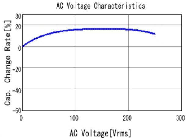
■ GA355DR7GB223KW01 C-AC Voltage capchange, DCOV, 25.0d
