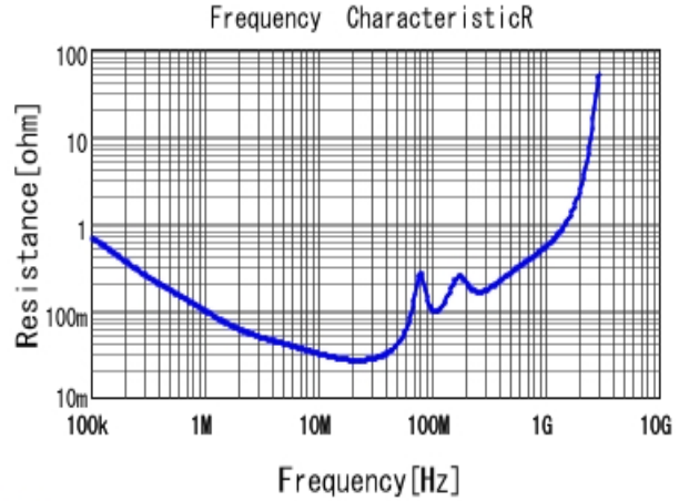
■ GA355DR7GB223KW01 R DCOV, 25degC
