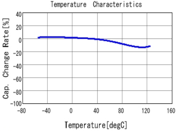
■ GA355DR7GB223KW01 C-Temp. capchange, DCOV, AC1Vrms
