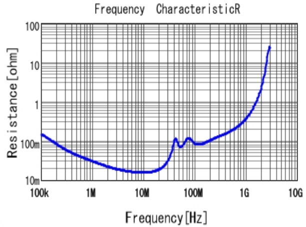
■ GA255DR7E2104MW01 R DCOV, 25degC
