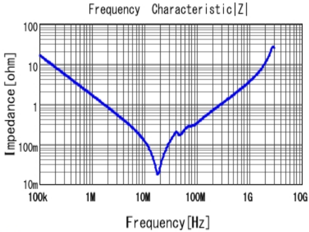
■ GA255DR7E2104MW01 |Z| DCOV, 25degC
