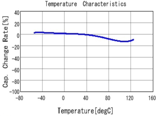
■ GA255DR7E2104MW01 C-Temp. capchange, DCOV, AC1Vrms
