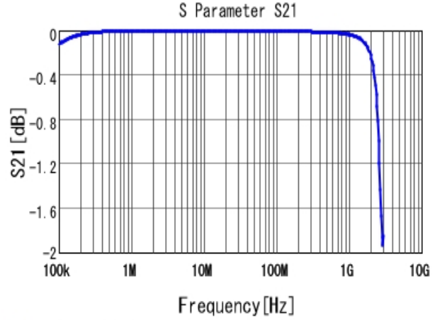
■ GA255DR7E2104MW01 S21 DCOV, 25degC
