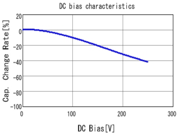
■ GA255DR7E2104MW01 C-DC bias capchange, 25.0degC, AC1V
