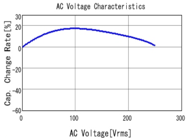
■ GA255DR7E2104MW01 C-AC Voltage capchange, DCOV, 25.0d
