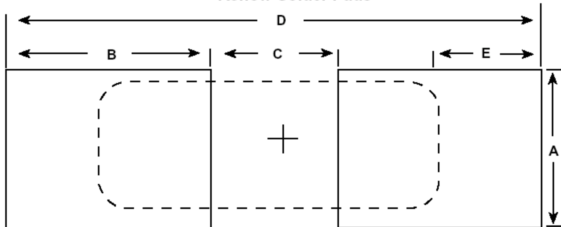
Reflow Solder Pads
