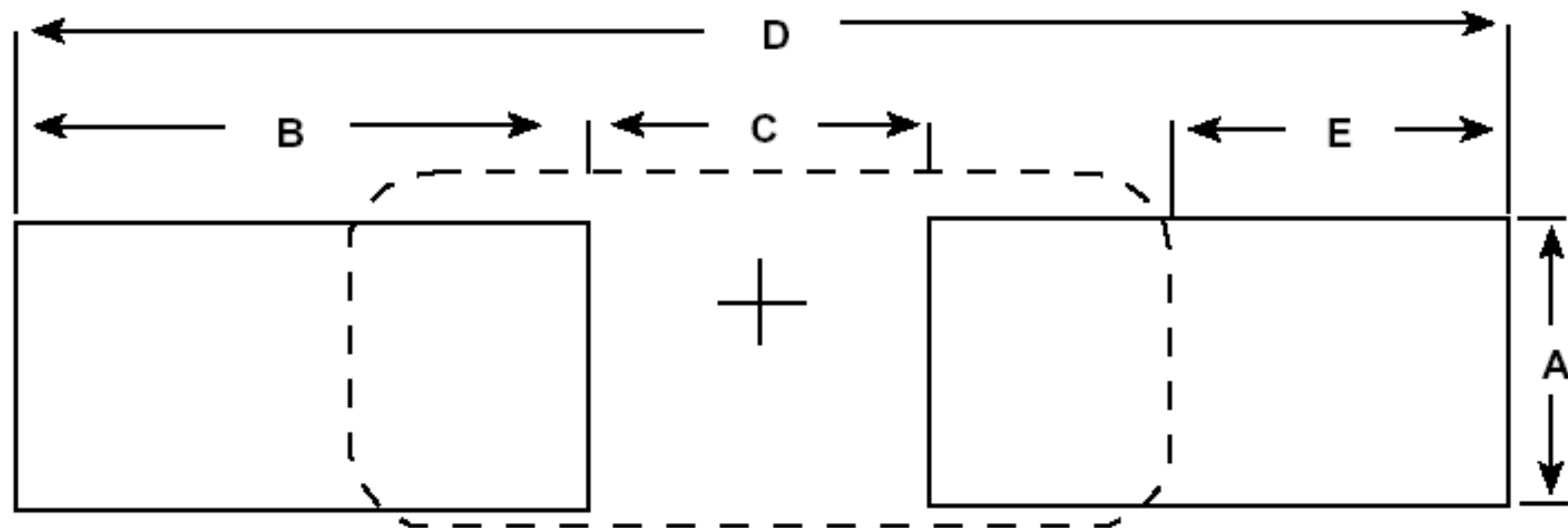
Wave Solder Pads
