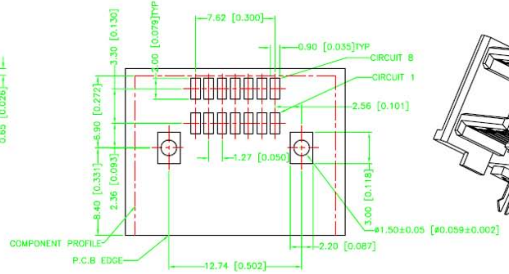
P.C.B LAYOUT COMPONENT SIDE
