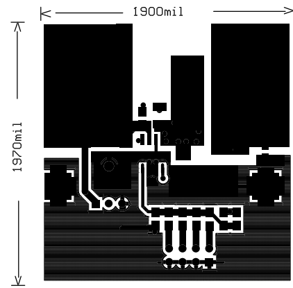
Figure 7b. Top Side Copper
