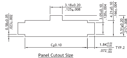
Panel Cutout Size
