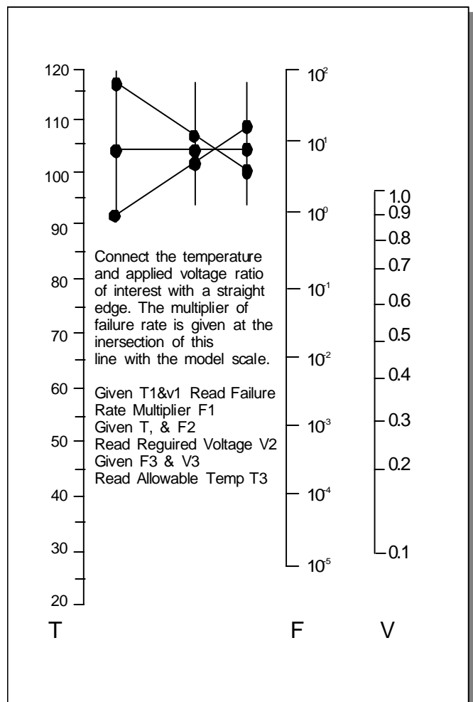
Fig.8 Reliability Nomograph
