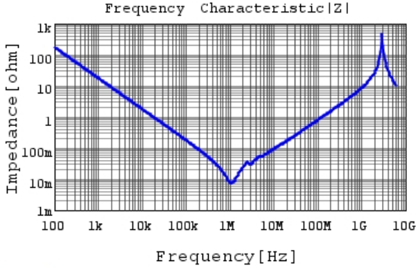
KRM55TR72A106MH01 |Z| DCOV, 25degC
