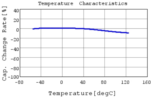
■ KRM55TR72A106MH01 C-Temp. capchange, DCOV, 1
