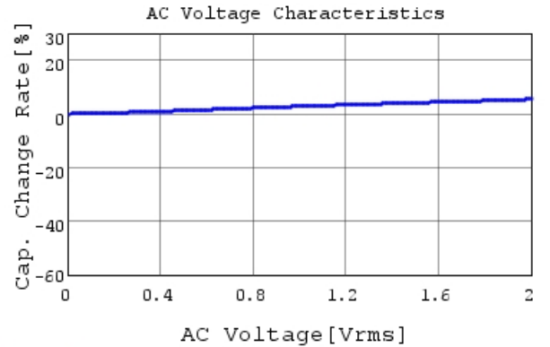
KRM55TR72A106MH01 C-AC Voltage capchange, Dc
