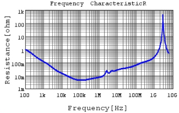
KRM55TR72A106MH01 R DCOV, 25degC
