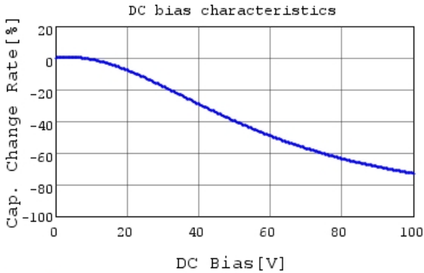
KRM55TR72A106MH01 C-DC bias capchange, 25.0c
