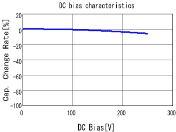
■ GA355DR7GF472KW01 C-DC bias capchange, 25.0degC, AC1V
