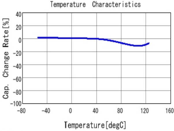
■ GA355DR7GF472KW01 C-Temp. capchange, DCOV, AC1Vrms
