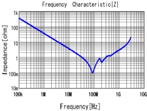
■ GA355DR7GF472KW01 |Z| DCOV, 25degC
