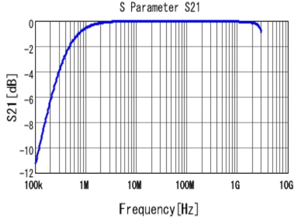
■ GA355DR7GF472KW01 S21 DCOV, 25degC
