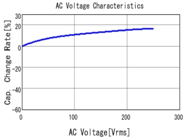
■ GA355DR7GF472KW01 C-AC Voltage capchange, DCOV, 25.0d
