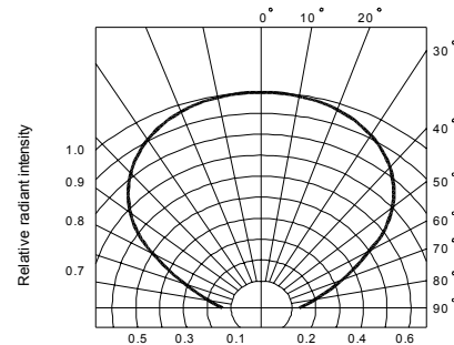
Fig.6 Radiation diagram
